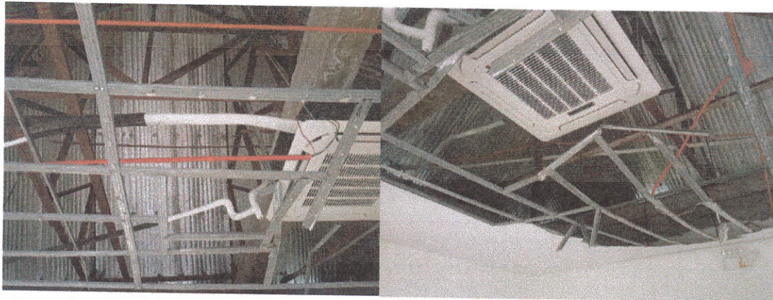
Damaged gypsum ceiling at galleries for replacement
